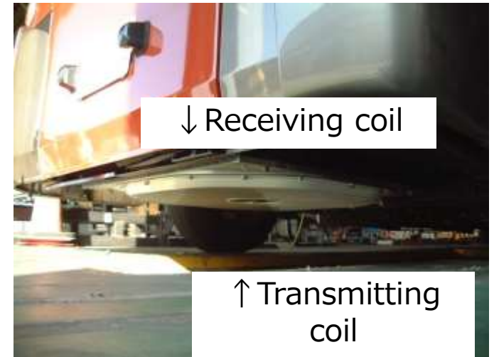
e.g.) WPT Coil for Parking Electric Bus
